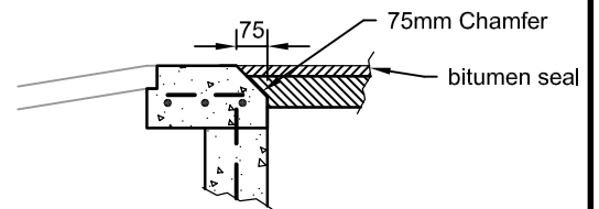
Detail for Bitumen Road
